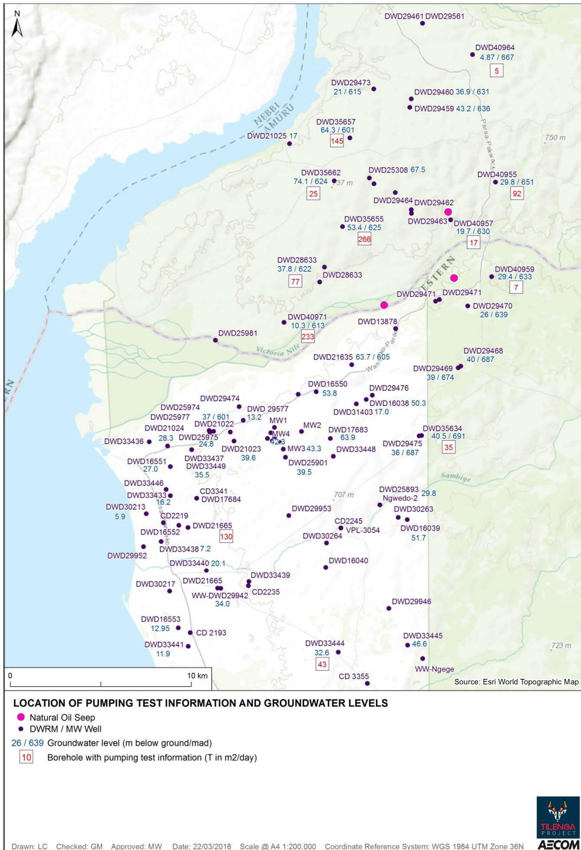
Figure 9-9: Locations of pumping test information and recorded groundwater levels
