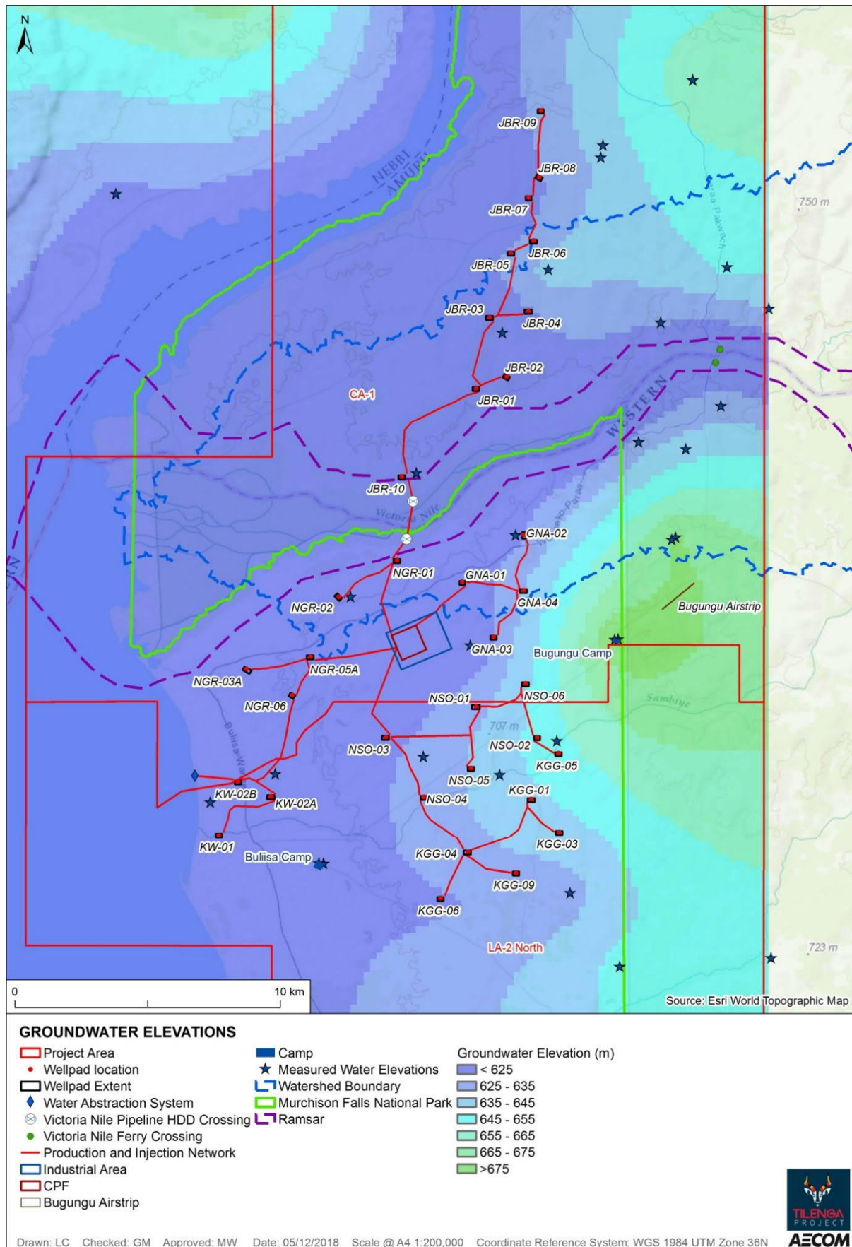
Figure 9-11: Groundwater Elevation across the Study Area
