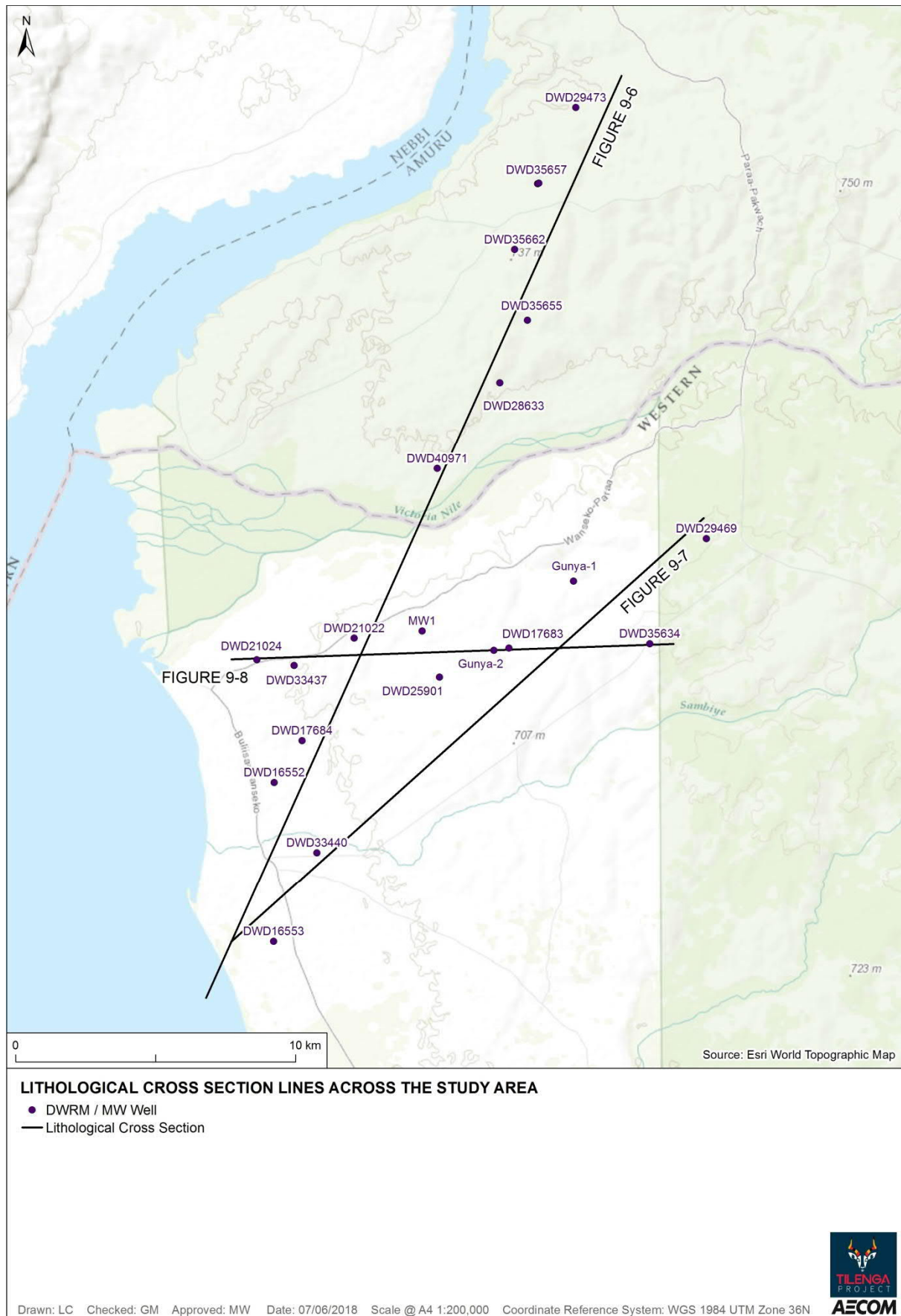
Figure 9-5: Lithological Cross Sections lines across the Study Area
