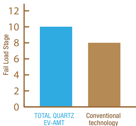
Gear durability: FZG A10/16,6R/90
