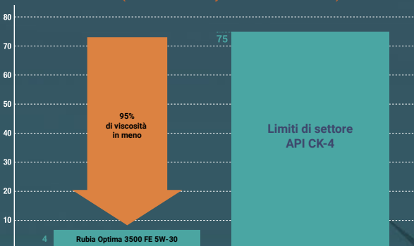
% Volvo T13 Test (KV 40 Viscosity Increase 300 360h)
